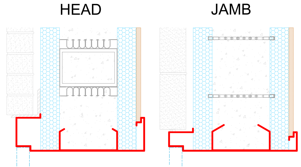
IFA Door Solution
