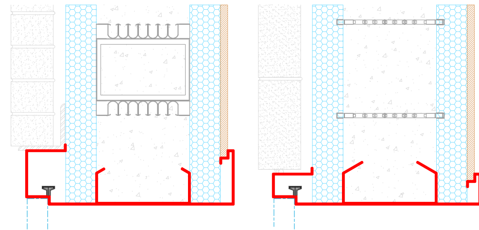
Thermally Broken IFA Door Solution
