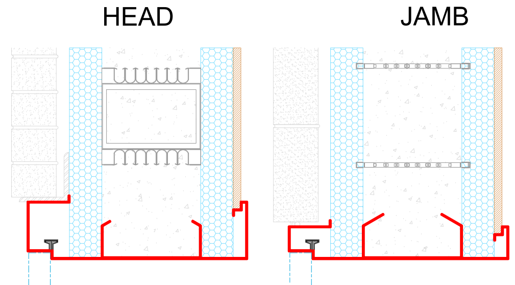
Thermally Broken IFA Door Solution
