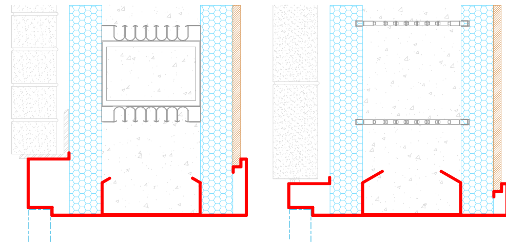
IFA Door Solution
